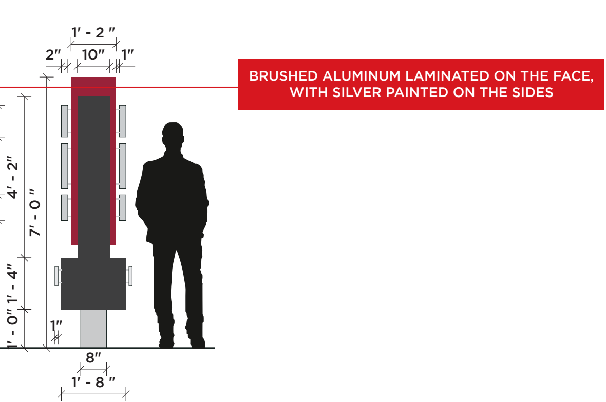
SIDE VIEW
